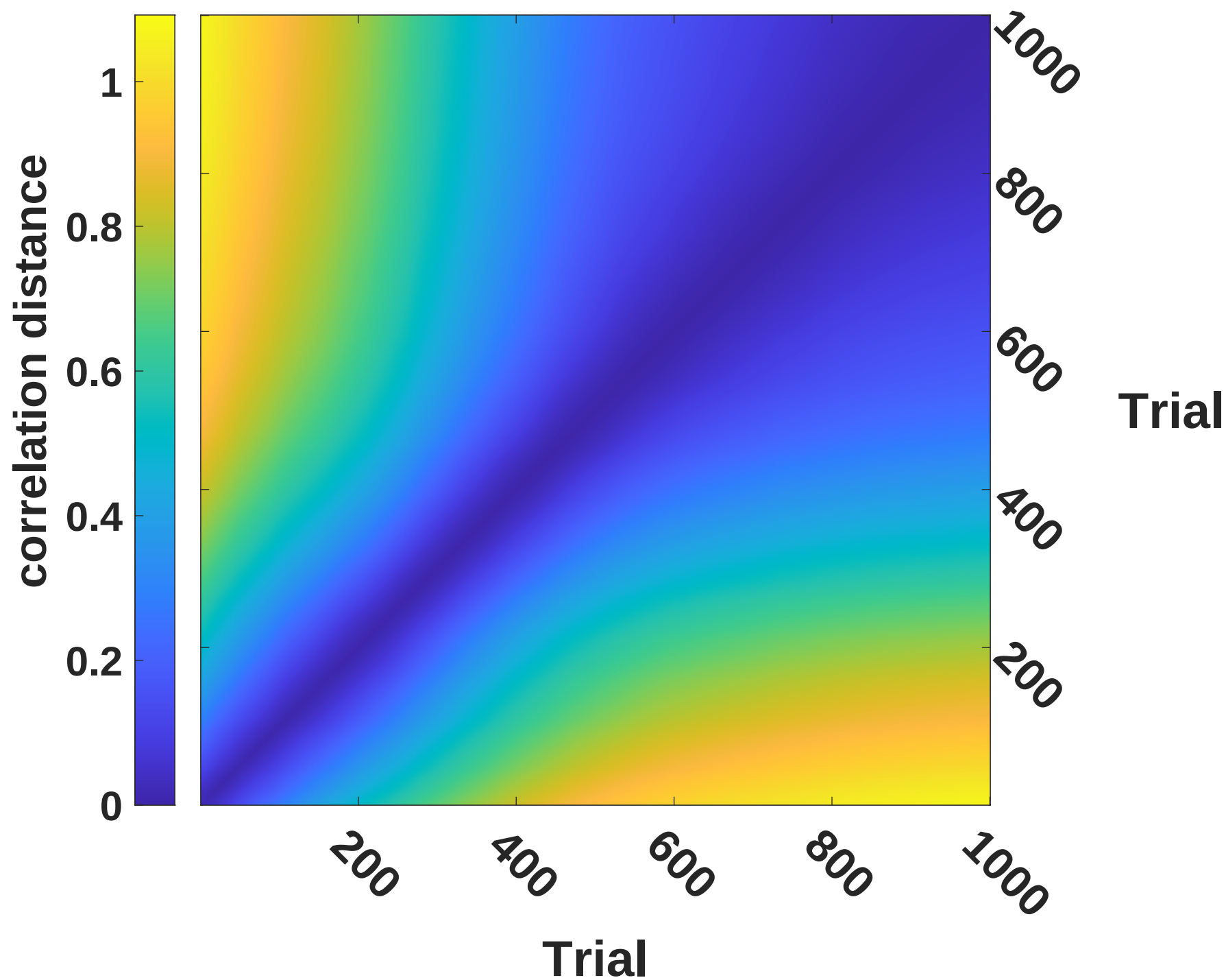
spike counts Distance Matrix Averaged on 40 Simulations
